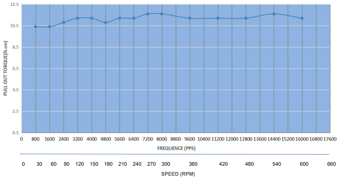
PULL OUT TORQUE CURVE OF 14HS11-1004S
