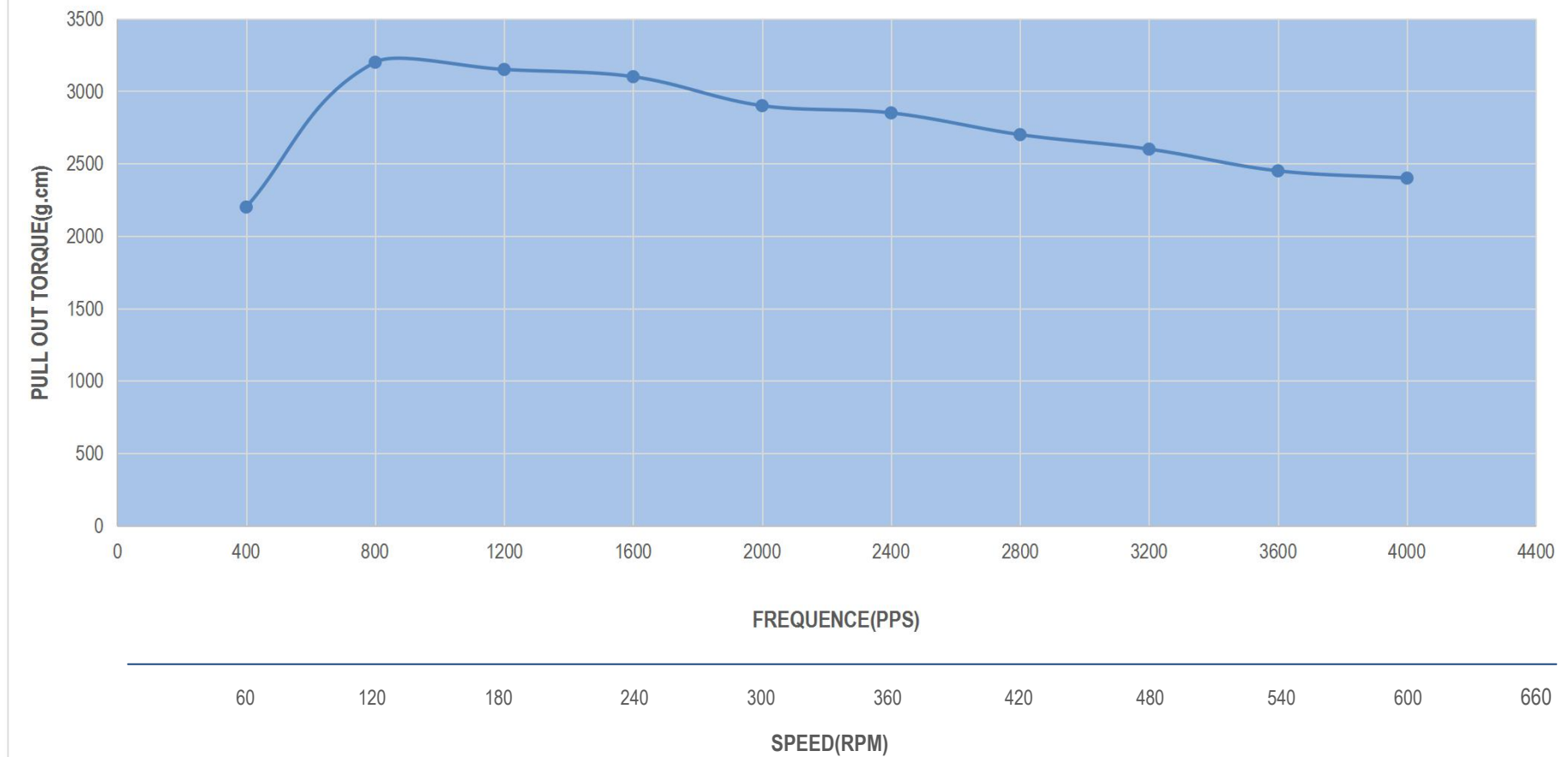
14HS20-1504S PULL OUT TORQUE(1.5A/P 24V HALF STEP /CONSTANT CURRENT)
