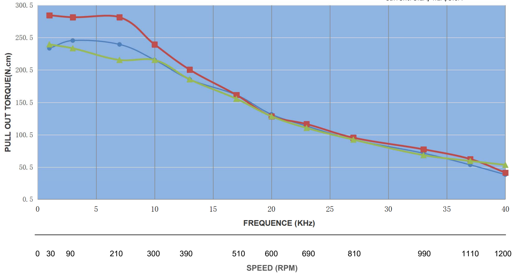
PULL OUT TORQUE CURVE OF 23HS45-4204D
