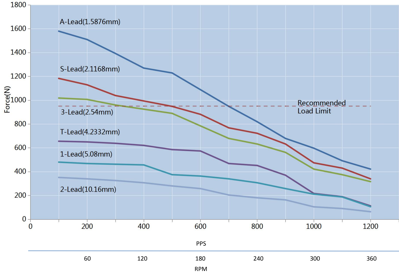
Nema 23 linear steppers double stack(24V)
