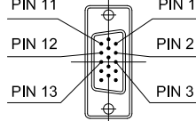
4-PIN GX16 FEMALE PLUG 15-PIN DB MALE PLUG
