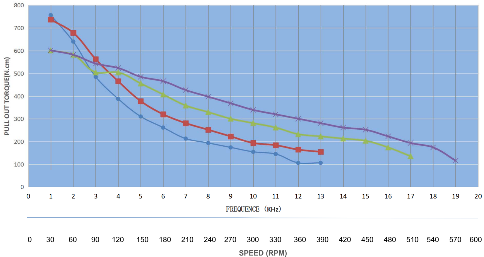
PULL OUT TORQUE CURVE OF 34HS38-3008S
