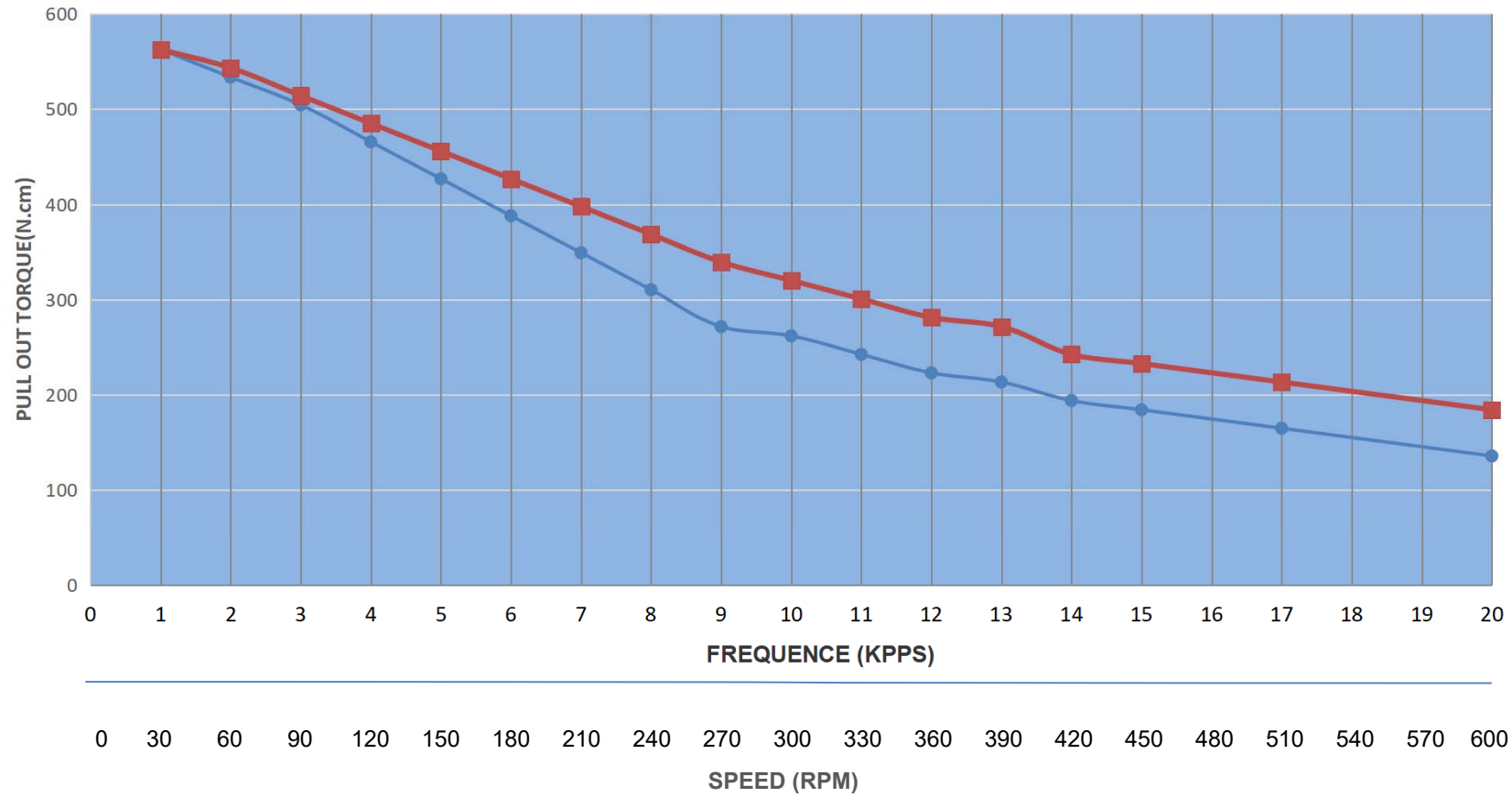
PULL OUT TORQUE CURVE OF 34HS38-4204D
