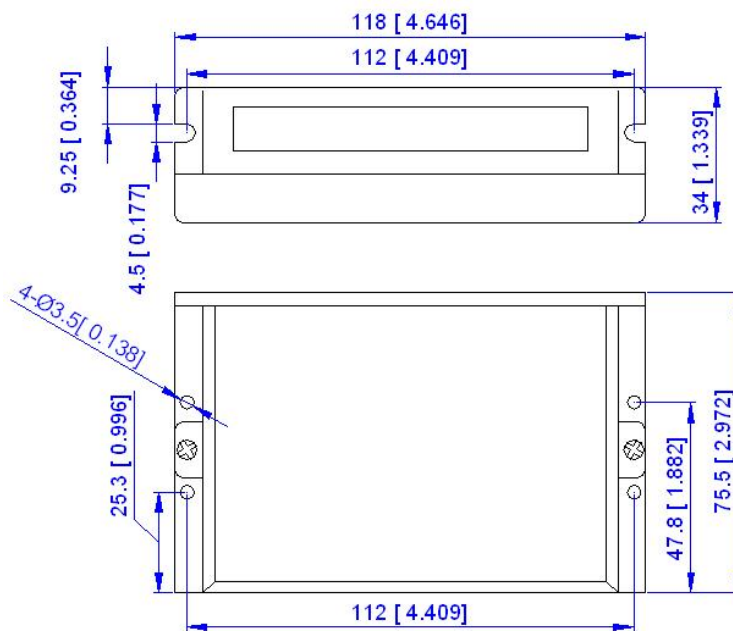
Figure 1 Mechanical specifications
